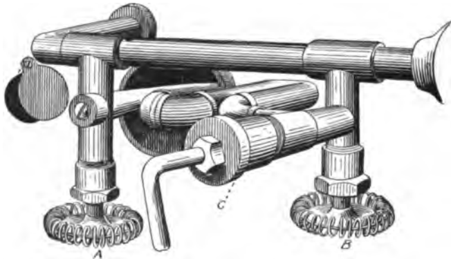
FIG. 218.—Showing the torch in position. By reference to Fig. 217, it may be readily understood that the head of the torch, C, is attached to a nipple on B by screw, G; the bent tube being thrust through a port in the burner casing so as to come directly over the fire; the nozzle entering the mixing tube by the side of the nozzle on the main valve, A.
